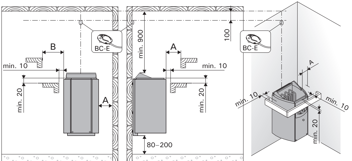
Safety distances (all dimensions in millimeters)
