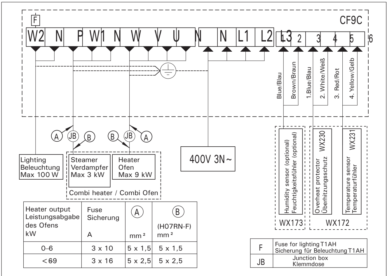
Electrical connections for the heaters, as well as for the control unit CF9C
