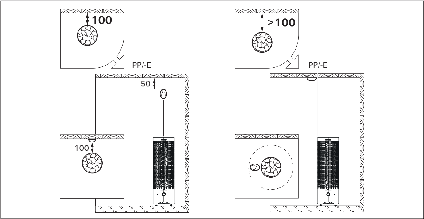
Installing the sensor (all dimensions in millimeters)
