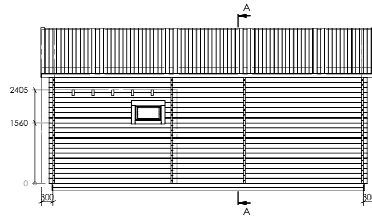
Facade B-A
