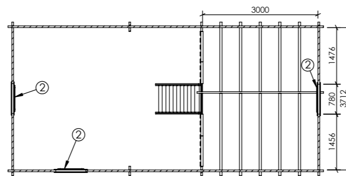
Plan II
