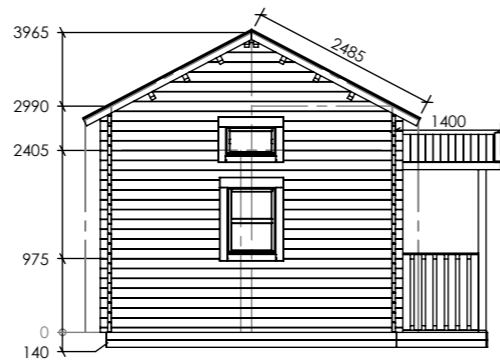
Facade 3-1
