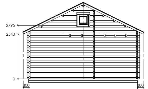
Facade C-A
