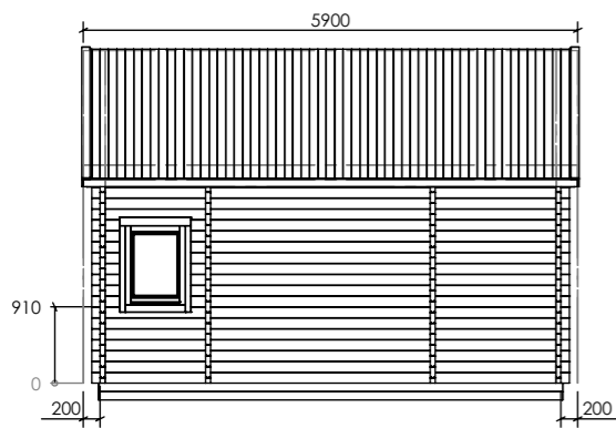
Facade 4-1
