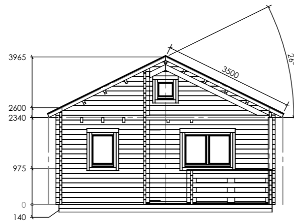
Facade A-C
