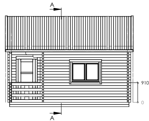
Facade 1-4
