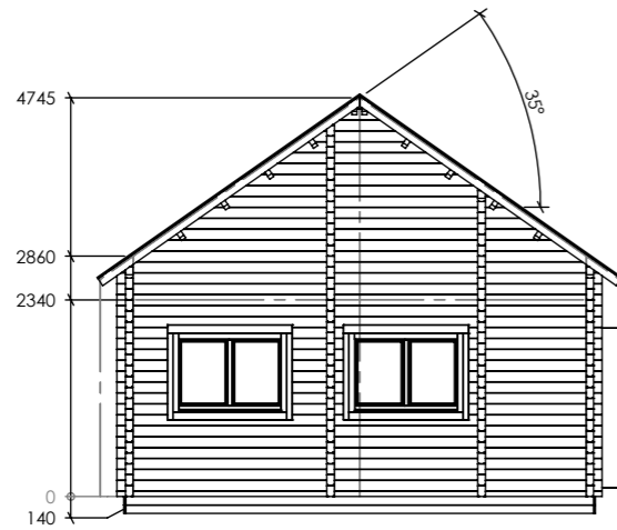
Facade 1-4
