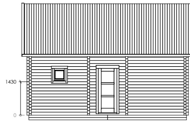
Facade D-A
