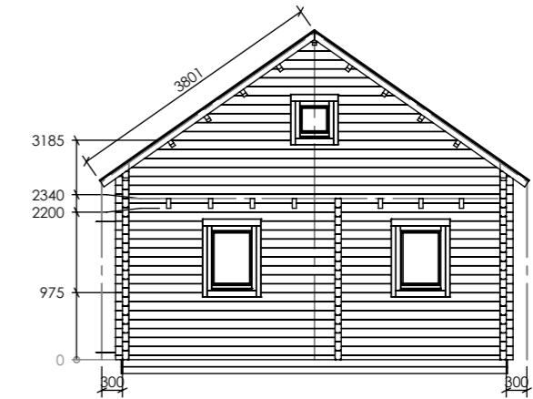
Facade 4-1
