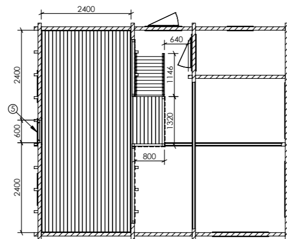
Plan II
