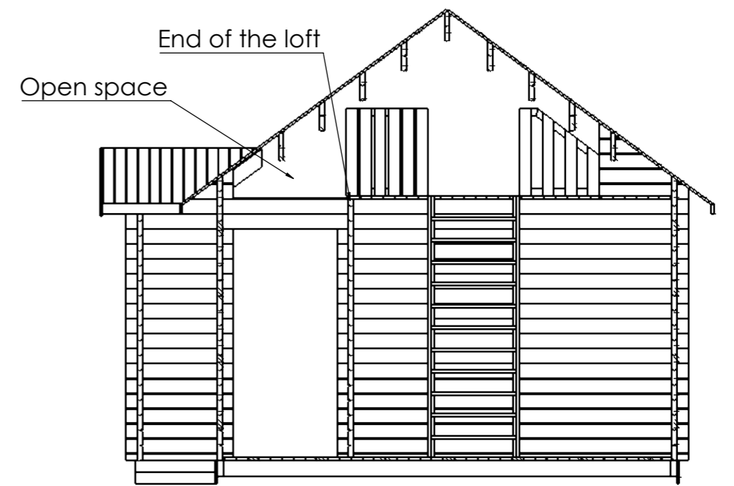
SECTION U-U
