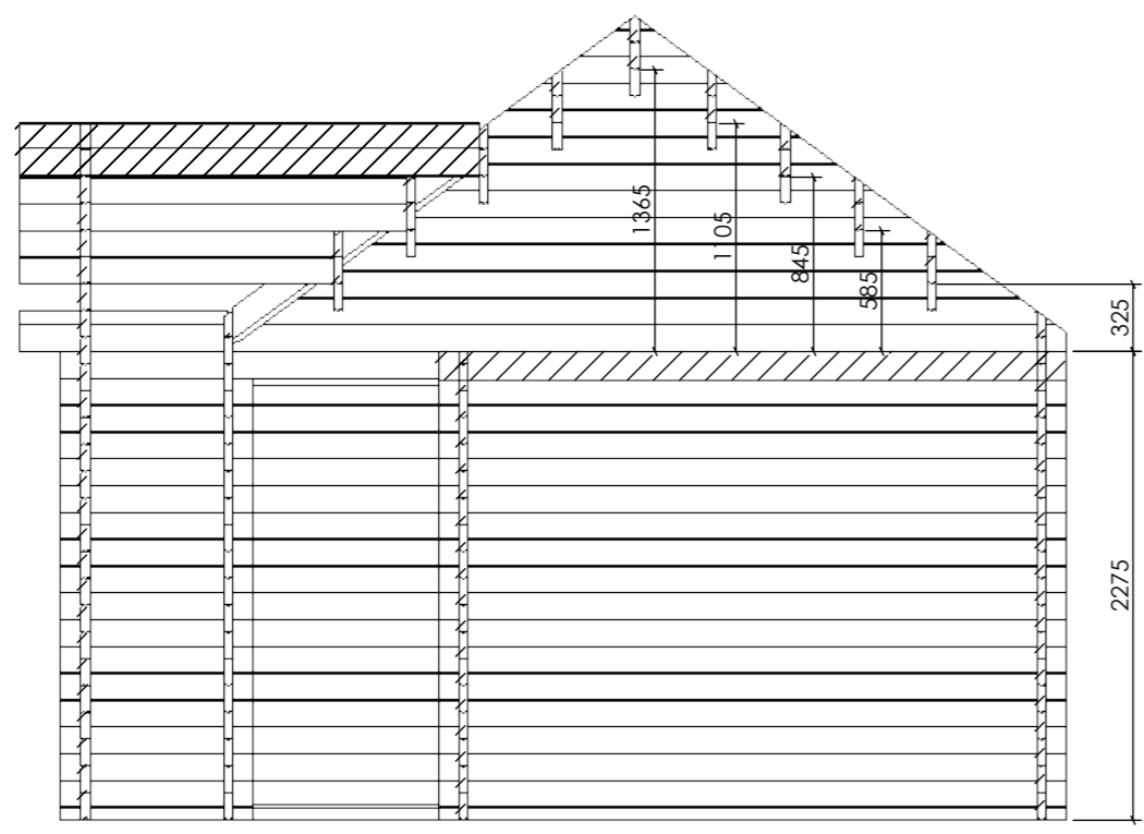
SECTION T-T
